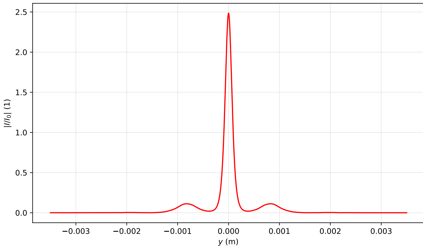
Intensity profile I(x=0, y, z=1.911)/I_0 , P_{in}=8.0P_{cr} , artificial time
